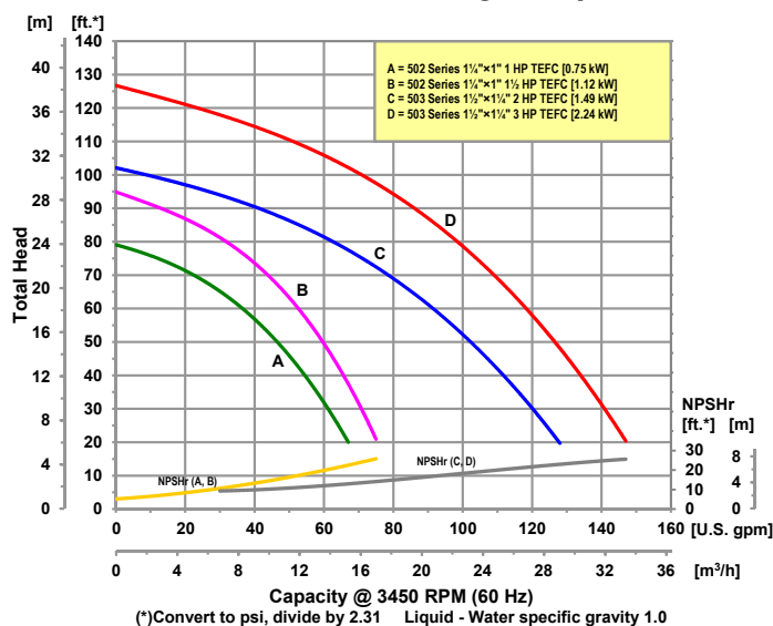
Performance of Centrifugal Pumps
