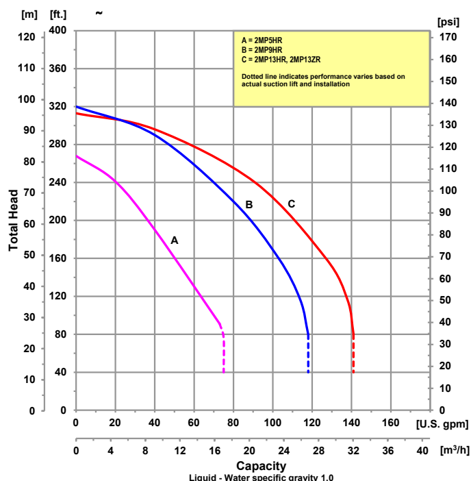
Performance of Engine-Driven 2-Stage High Pressure Pumps
