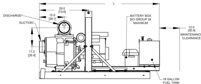
Skid Model
