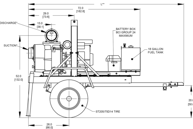
Trailer Model
